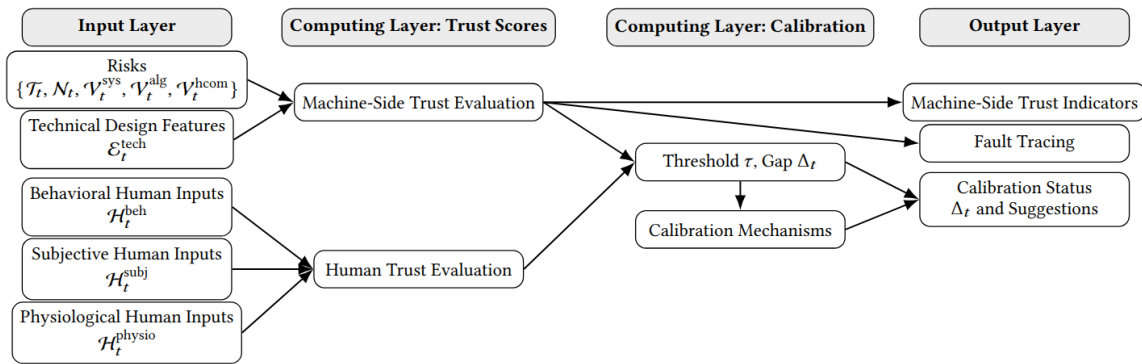
Fig. 1. CRiDiT Blueprint
