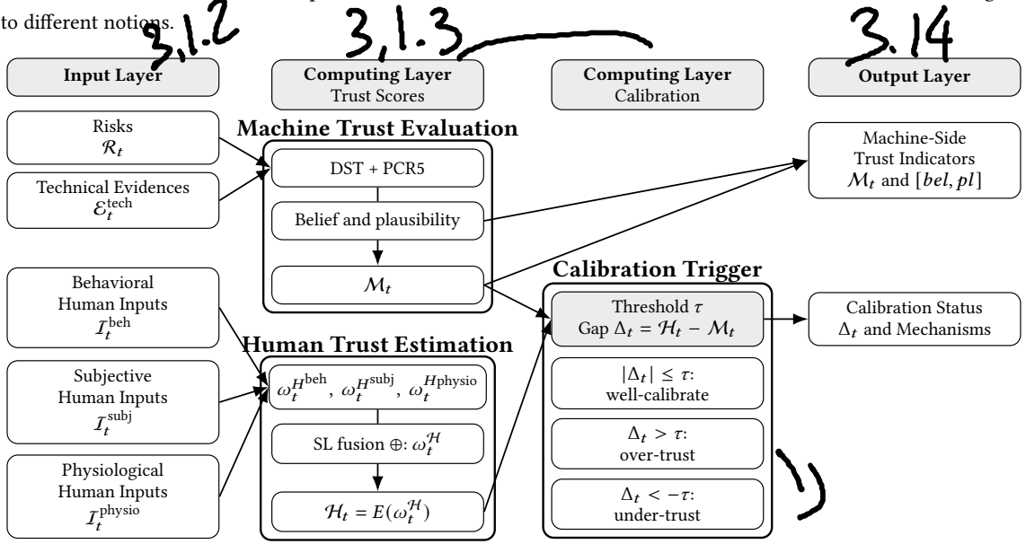
Fig. 2. CRiDiT Overview
