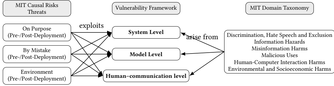
Fig. 3. Relation between MIT Causal Taxonomy [19], Operational Vulnerability Framework, and MIT Domain Taxonomy [17]
