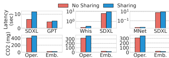
Fig. 3. Sharing GPUs can lead to increased net carbon emissions compared to dedicating a GPU per model. See § 3 Q2.
