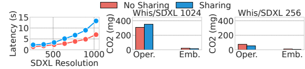
Fig. 6. CO2 for SDXL/Whisper when SDXL generates 1K×1K resolution images vs. 256×256. Input/output requirements impact spatial sharing's efficacy in reducing emissions. See § 3 Q3.
